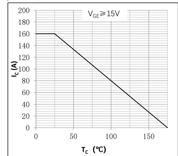
● Fig.6 Continuous collector current as a function of case temperature; Calculative values
